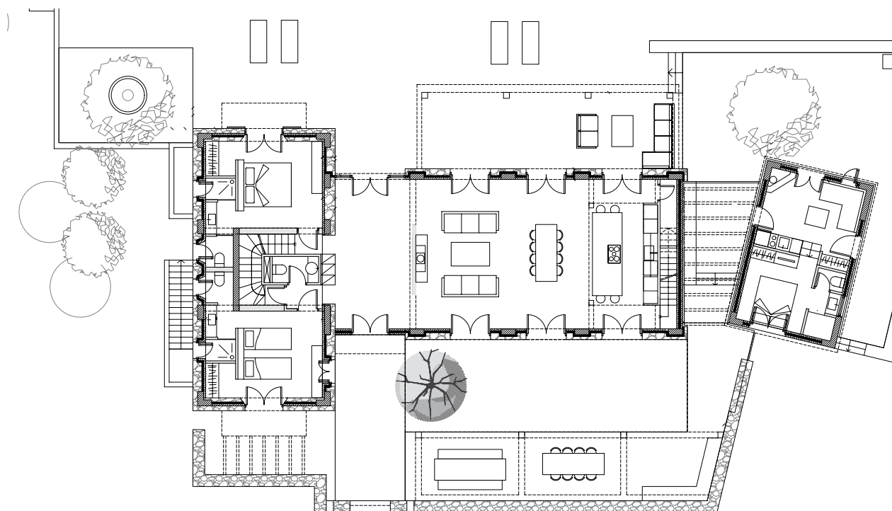
ΚΑΤΟΨΗ GROUND FLOOR PLAN
